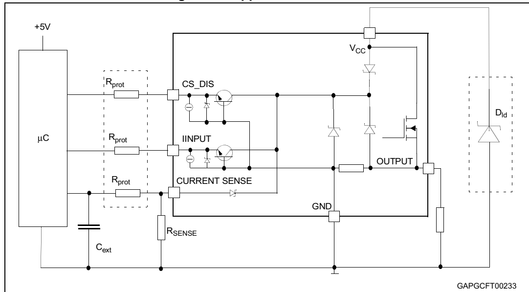
Figure 22. Application schematic
