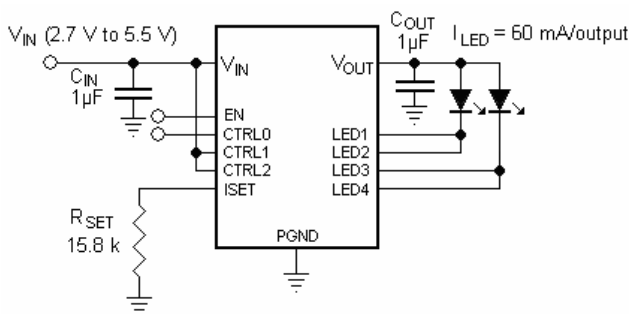
Figure 5. Application circuit with one LED
