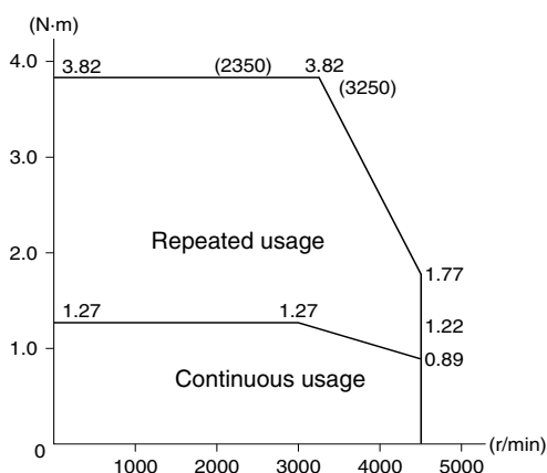
R7M-AP40030 (400 W)
