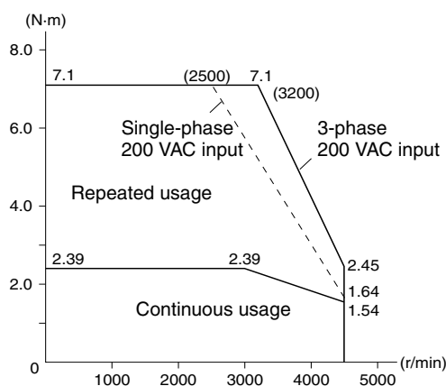
R7M-AP75030 (750 W)
