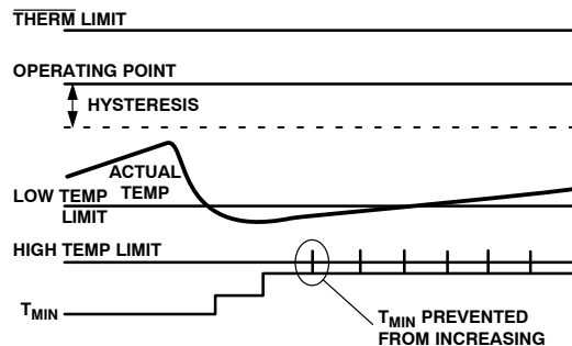
Figure 73. T_{MIN} Adjustments Limited by High Temperature Limit
