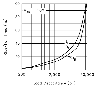
FIGURE 8. RISE/FALL TIME vs LOAD
