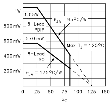
FIGURE 1. MAX POWER DERATING CURVES
