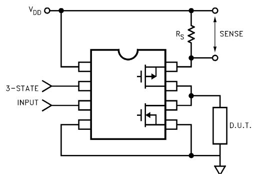
FIGURE 9. PIN DRIVER
