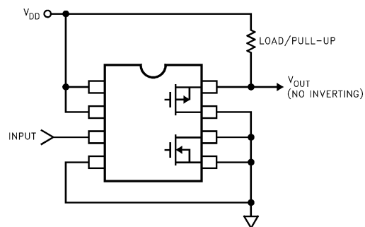
FIGURE 12. PMDS FOLLOWER
