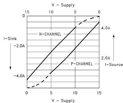
FIGURE 4. PEAK DRIVE vs SUPPLY VOLTAGE
