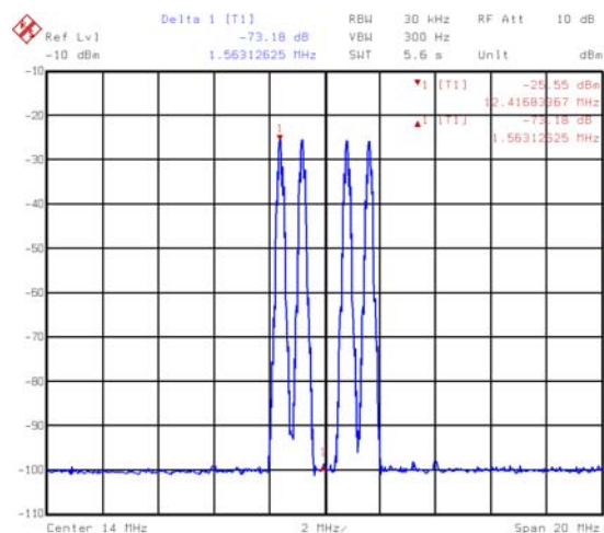
FIGURE 6. FOUR GSM CARRIERS AT 12.4-15.6MHz, 78MSPS (73dBc - 20MHz WINDOW, 6dB PAD)
