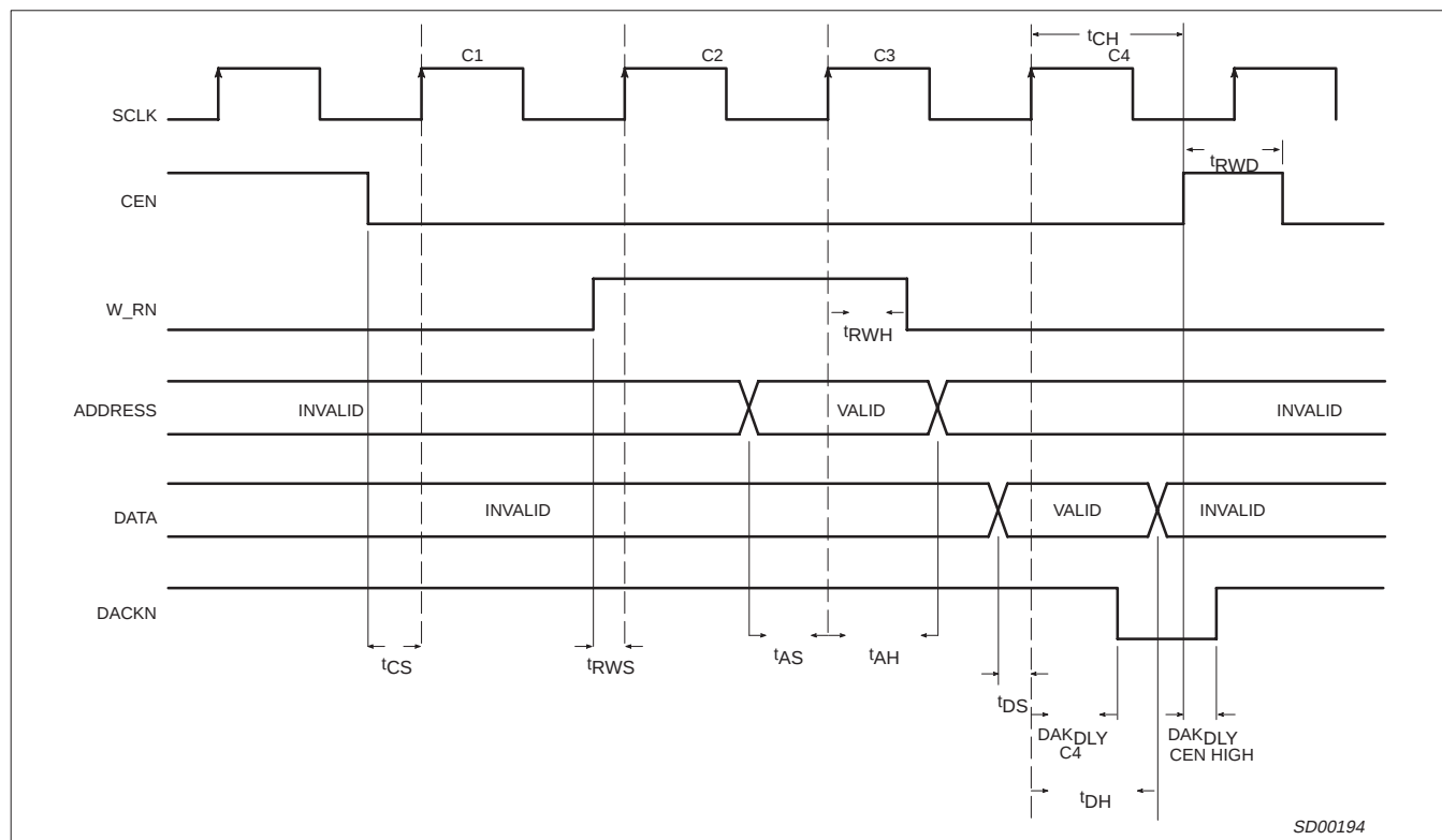
Figure 2. Basic Write Cycle, ASYNC
