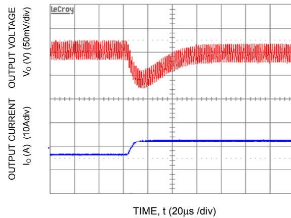
Figure 28. Transient Response to Dynamic Load Change from 50% to 100% at 12V in , C out -1x47μF+1x330μF, C Tune -2700pF & R Tune -330ohms
