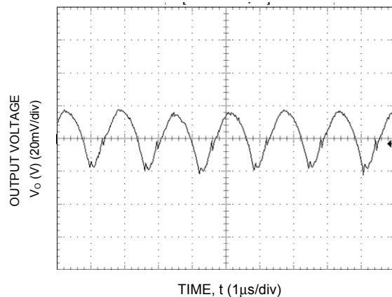
Figure 21. Typical output ripple and noise ( C_o=22\mu F ceramic, V_{IN} = 12V , I_o = I_{o,max} ).
