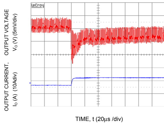
Figure 4. Transient Response to Dynamic Load Change from 50% to 100% at 12Vin, C_{out}=3 \times 47\mu\text{F} + 6 \times 330\mu\text{F} , C_{Tune}=47\text{nF} , R_{Tune}=180\Omega
