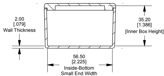
SECTION C-C Small End View
