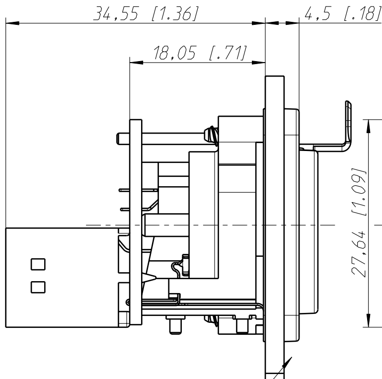
Frontplatte frontpanel
