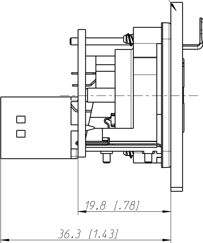
Frontplatte frontpanel
