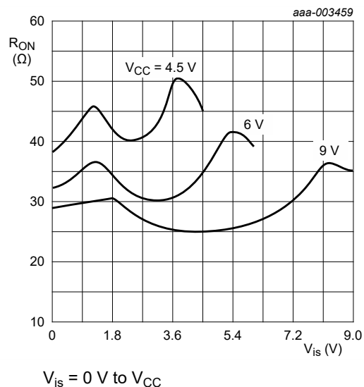
Fig. 9. Typical R_{ON} as a function of input voltage V_{IS}
