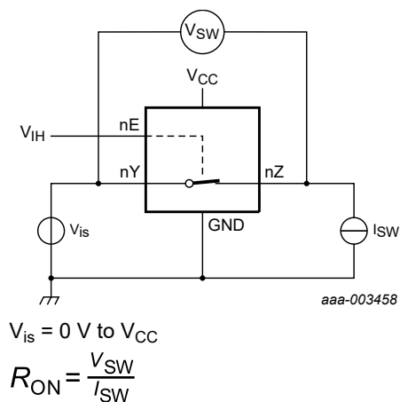
Fig. 8. Test circuit for measuring R_{ON}
