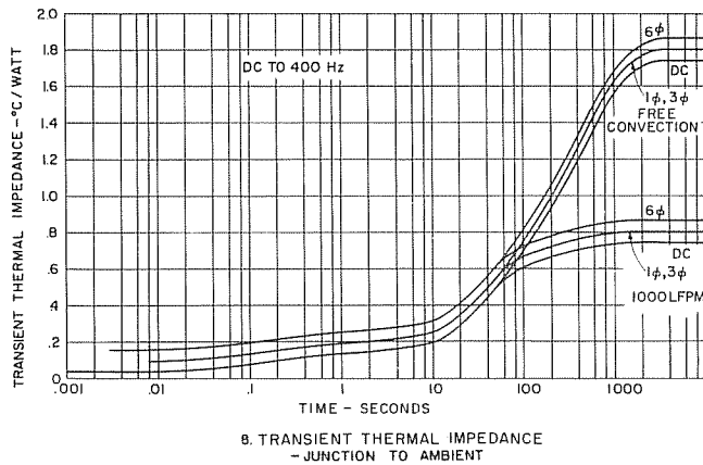
12. TRANSIENT THERMAL IMPEDANCE - JUNCTION-TO-AMBIENT
