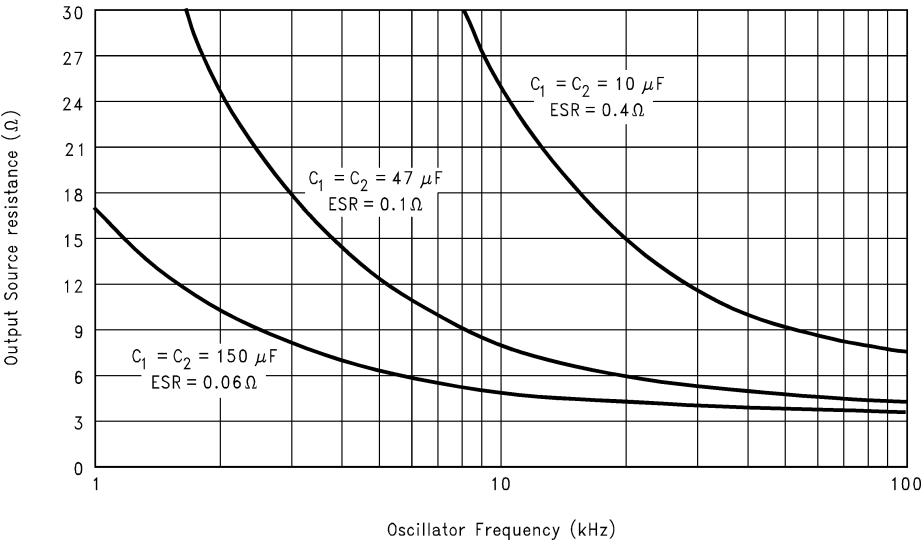
Figure 17. Output Source Resistance vs Oscillator Frequency
