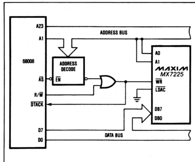
Figure 18. MX7225 to 68008 Interface, Single-Buffered Mode
