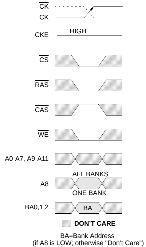
PRECHARGE Command
