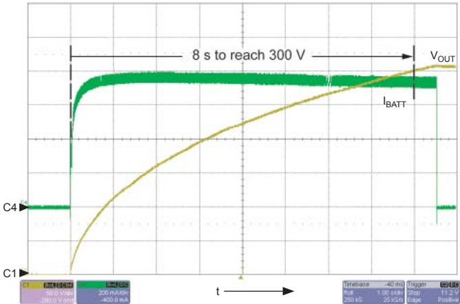
Charging Waveforms: 140 μF photoflash capacitor
