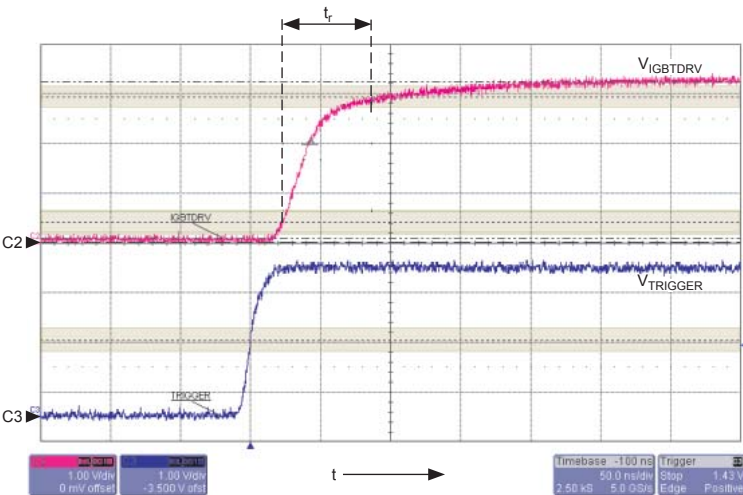
Rising Signal
