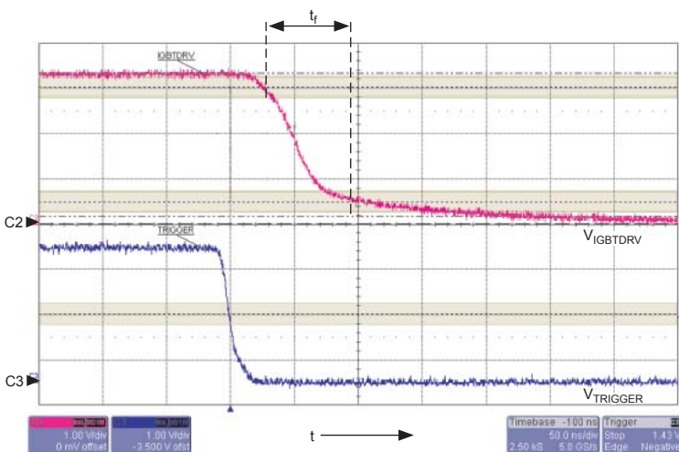
Falling Signal
