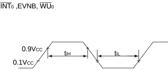
Figure 80 Interrupt Timing
