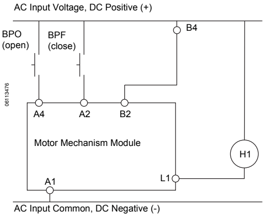
Figure 15: Motor Operator Without Overcurrent Switch Protection
