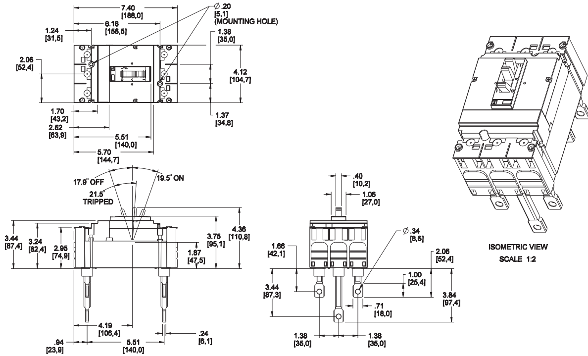
Figure 20: 15–150 A Rear Connected H-Frame 3P Circuit Breaker
