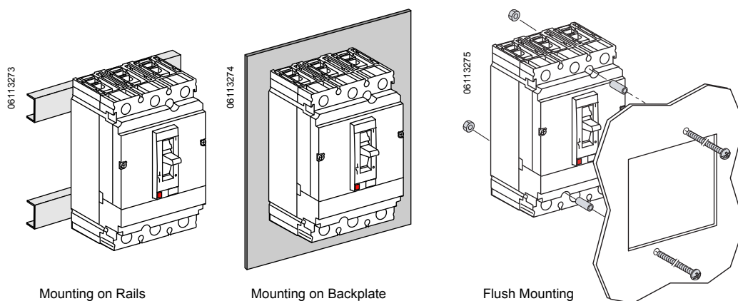
Figure 6: Unit-Mounting Options
