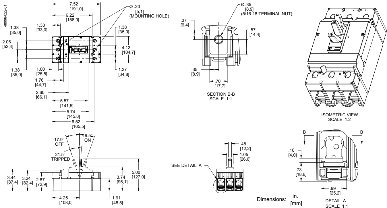
Figure 24: 150–250 A Lug-Lug J-Frame 3P Circuit Breaker
