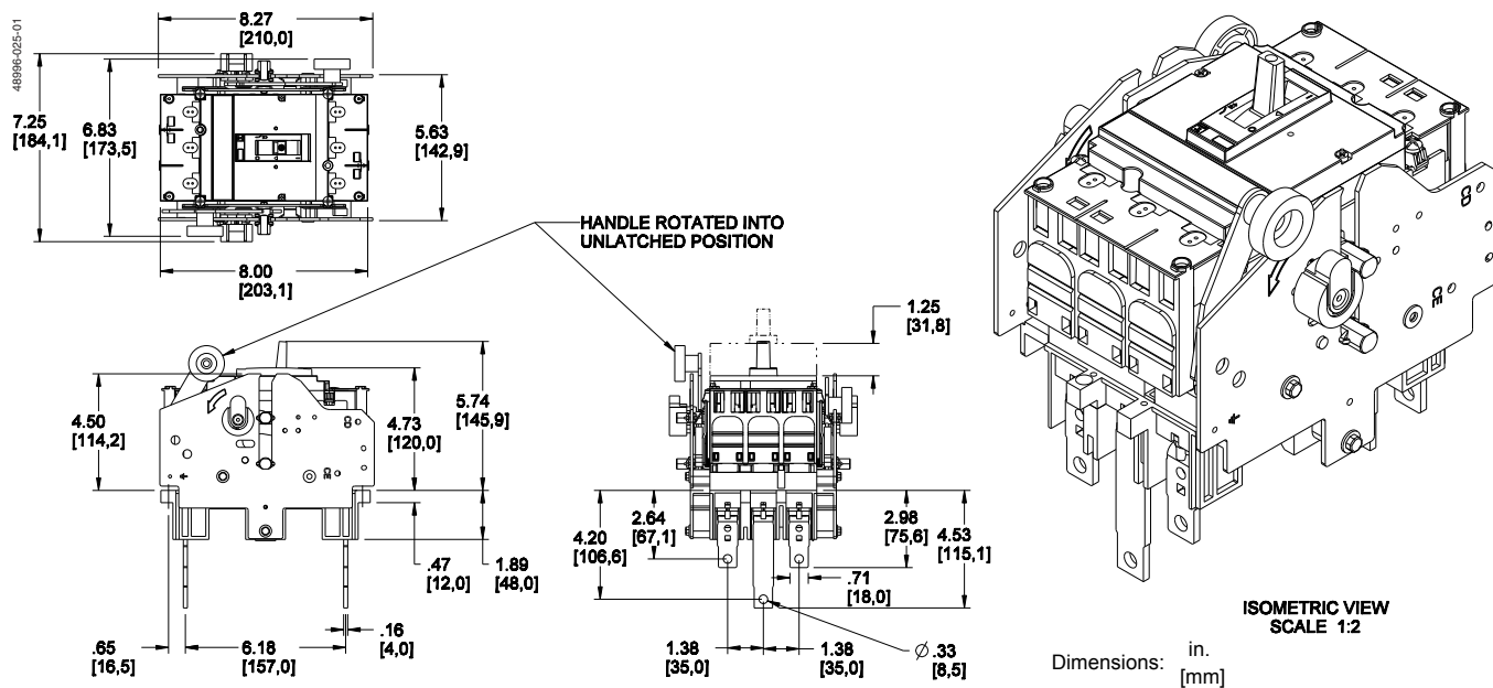
Figure 31: 15–250 A H- and J-Frame Drawout Circuit Breaker 3P Circuit Breaker
