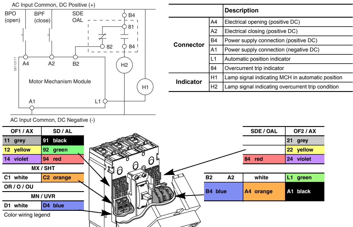
Figure 14: Standard Motor Operator Control Wiring
