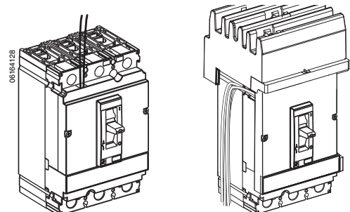
Figure 11: Accessory Connections
