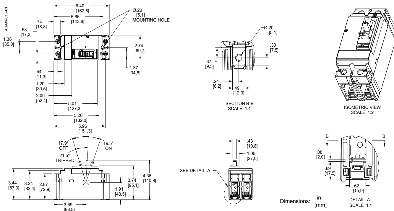
Figure 16: 15–150 A Bus Bar H-Frame 2P HD/HG Circuit Breaker
