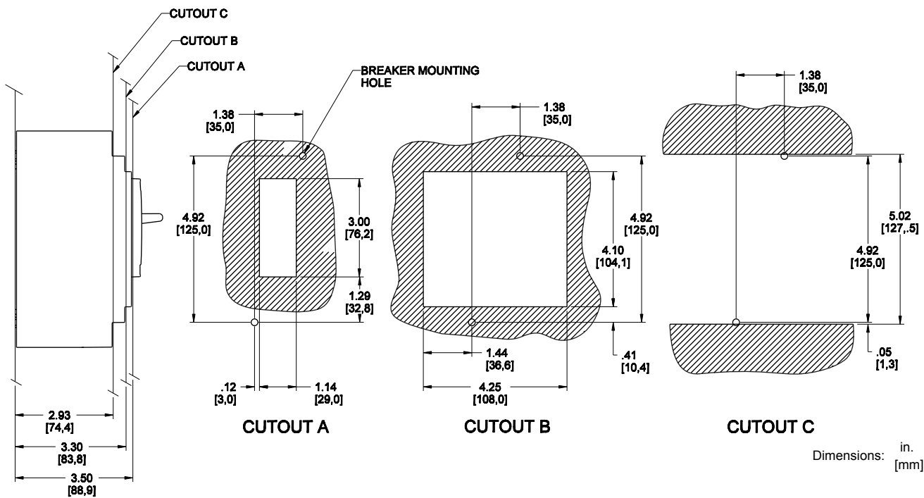
Figure 35: H and J-Frame Circuit Breaker Toggle Handle With Escutcheon Door Cutout
