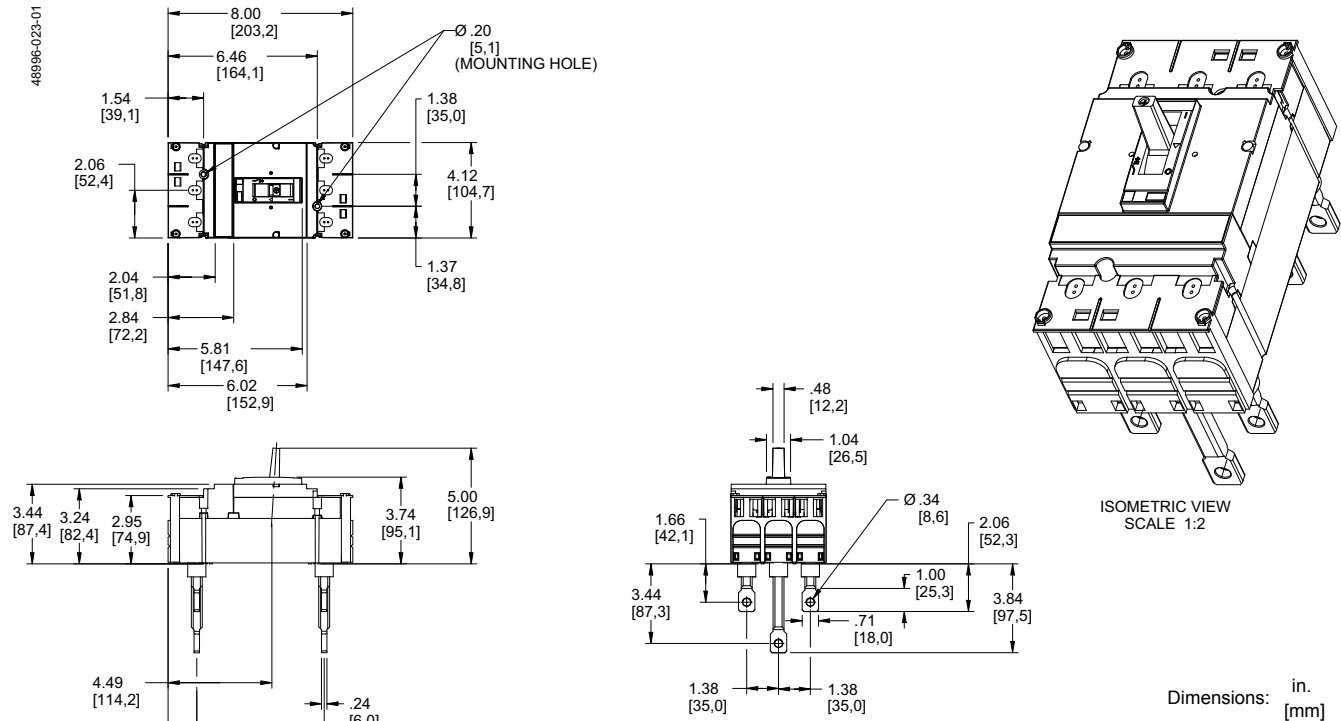
Figure 25: 150–250 A Rear Connected J-Frame 3P Circuit Breaker
