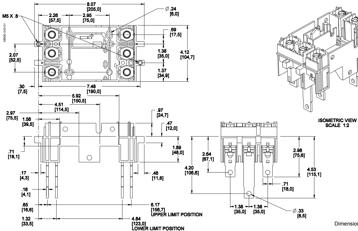
Figure 29: 15–250 A H- and J-Frame Plug-In Circuit Breaker 3P Circuit Breaker
