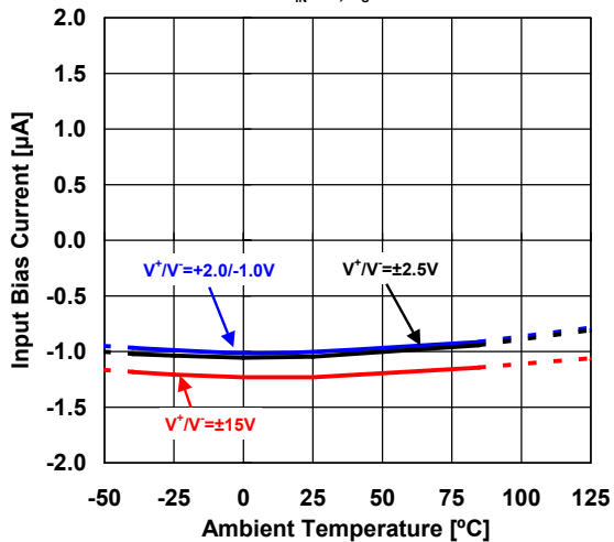
Input Bias Current vs. Temperature (Supply Voltage) V_{IN}=0\text{V} , R_S=50\Omega
