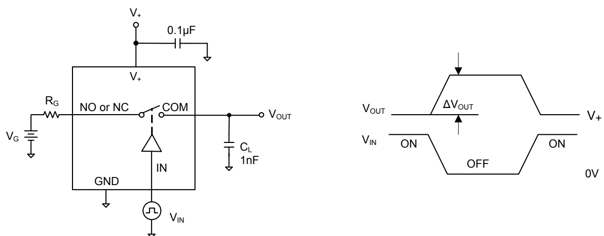
Test Circuit 3. Charge Injection
