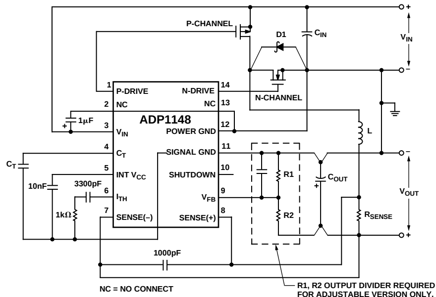
Figure 18. ADP1148 Layout Diagram (See Board Layout)
