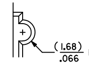
DETAIL "S"
