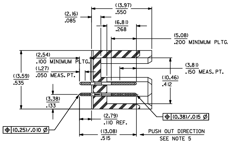
SECTION W-W
