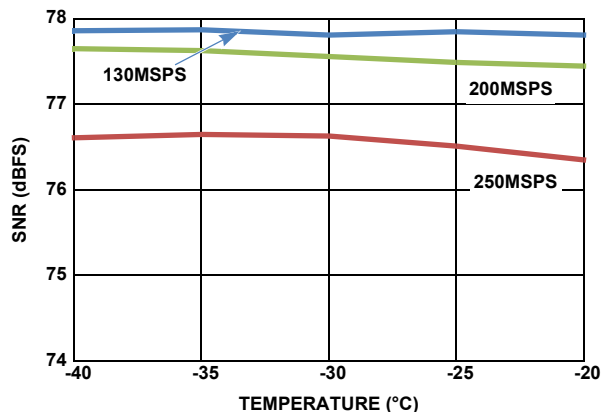
FIGURE 20. TYPICAL SNR PERFORMANCE vs TEMPERATURE, DEVICE CALIBRATED AT -40°C, f_{IN} = 105\text{MHz} , -2dBFS
