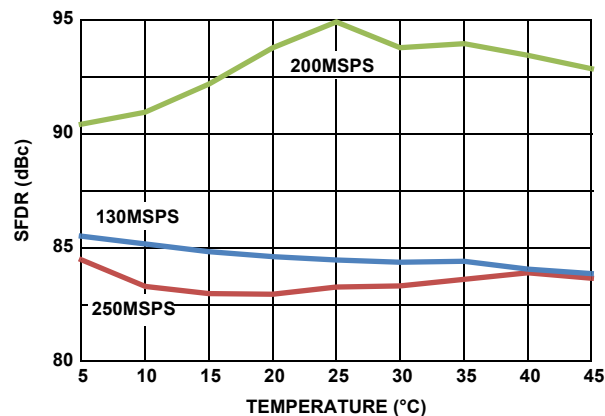
FIGURE 23. TYPICAL SFDR PERFORMANCE vs TEMPERATURE, DEVICE CALIBRATED AT +25 °C, f_{IN} = 105\text{MHz} , -2dBFS
