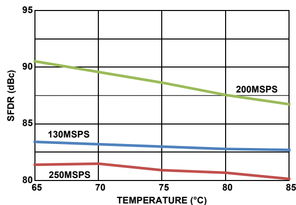
FIGURE 25. TYPICAL SFDR PERFORMANCE vs TEMPERATURE, DEVICE CALIBRATED AT +85 °C, f_{IN} = 105\text{MHz} , -2dBFS
