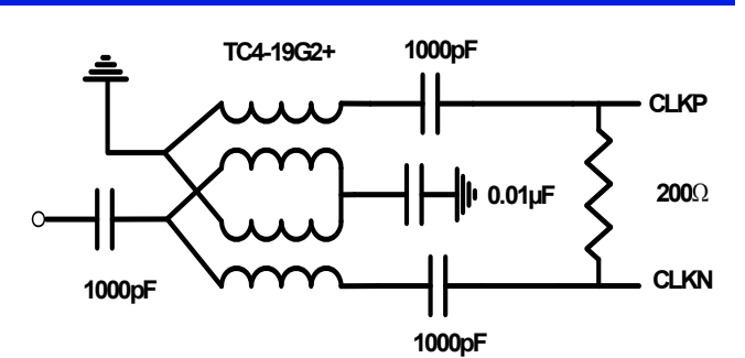
FIGURE 30. RECOMMENDED CLOCK DRIVE
