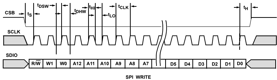
FIGURE 37. SPI WRITE
