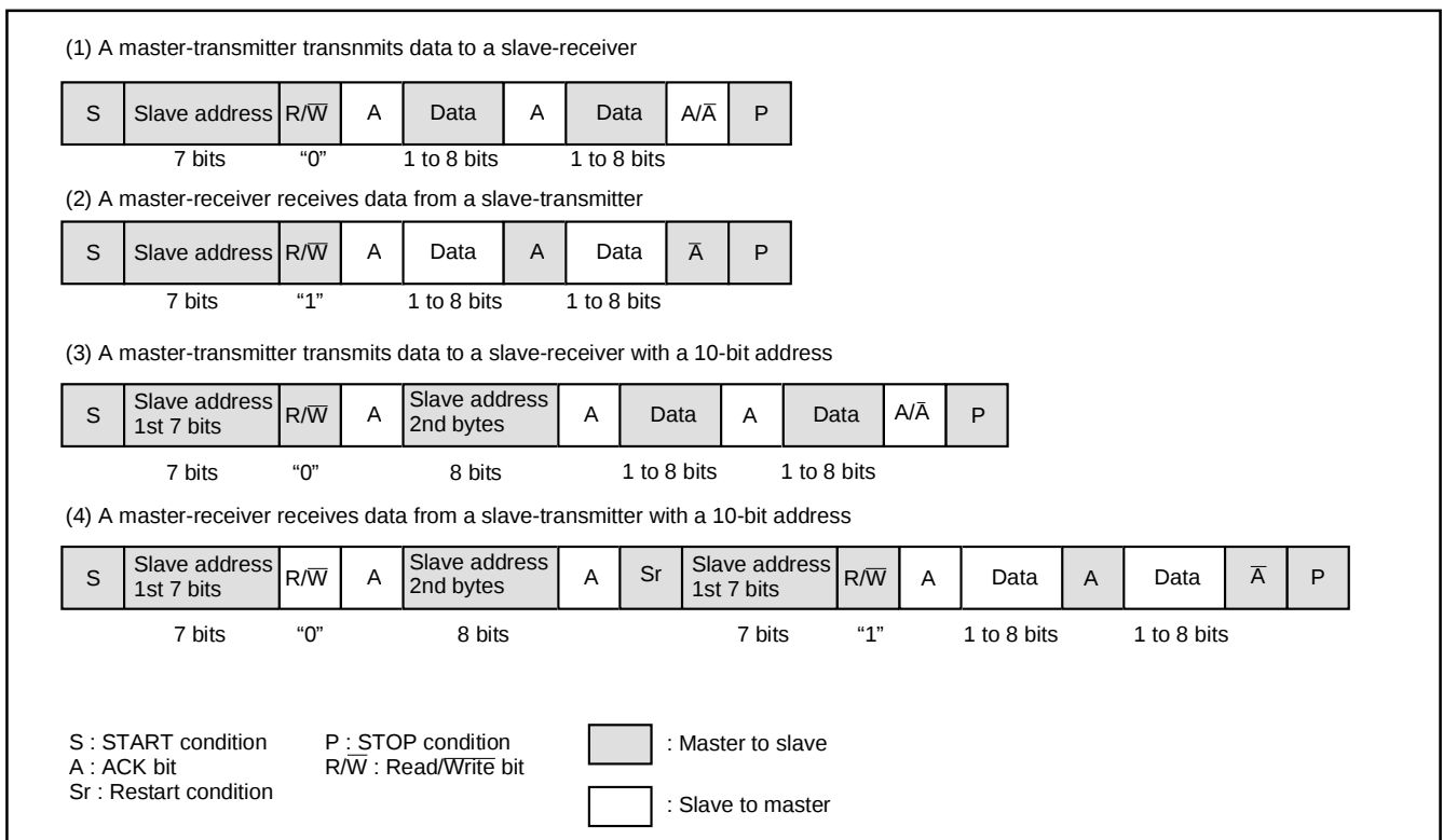
Fig. 39 Address data communication format
