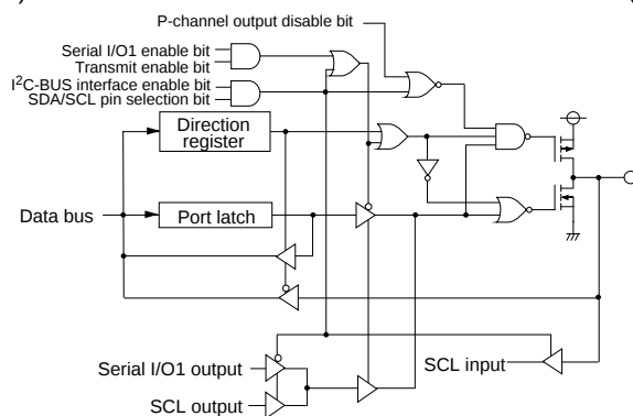
(11) Port P25
