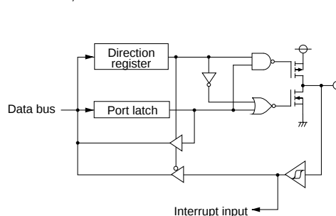
(16) Ports P41, P42
