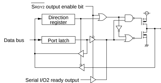
(4) Port P03
