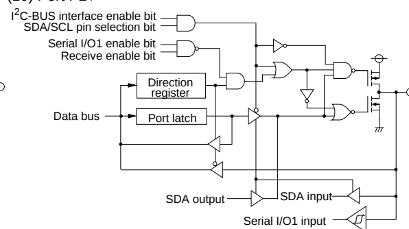
(10) Port P24
