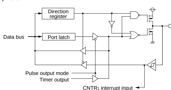
Fig. 11 Port block diagram (2)
