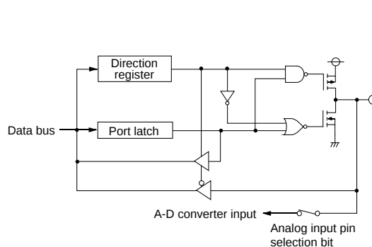
(14) Ports P30–P35
