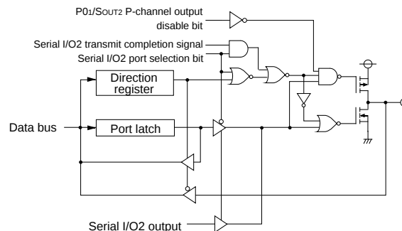
(2) Port P01
