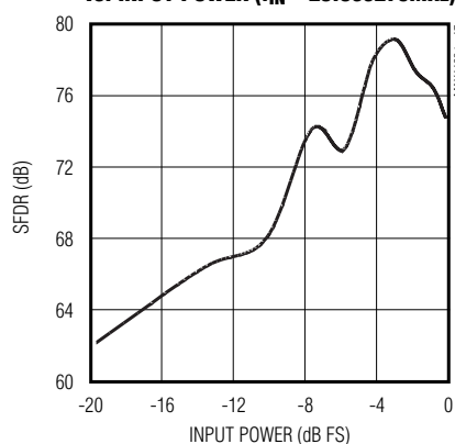
SPURIOUS-FREE DYNAMIC RANGE vs. INPUT POWER ( f_{IN} = 20.085279MHz )
