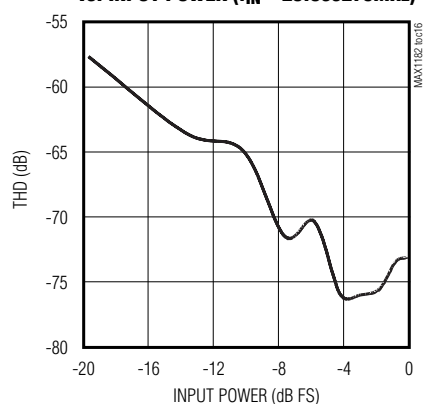
TOTAL HARMONIC DISTORTION vs. INPUT POWER ( f_{IN} = 20.085279MHz )
