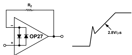
Figure 37. Pulsed Operation
