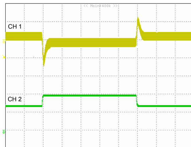
Figure 10: MGMT_PWR (3.3V) dynamic response (1mS/div):
