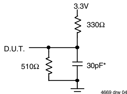
Figure 2. Output Load
