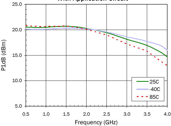
P1dB versus Frequency With Application Circuit
