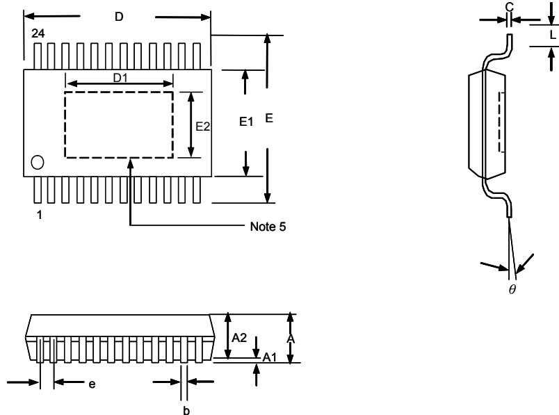
TSSOP-24 (FD) Package
