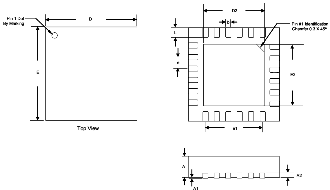
QFN4X4-24 Package
