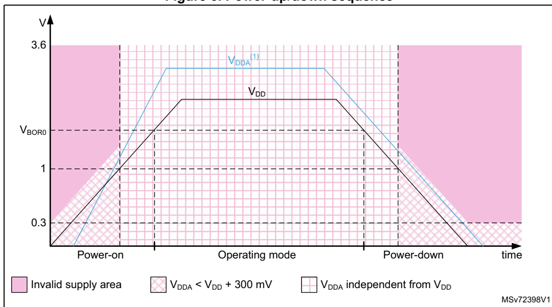
Figure 3. Power-up/down sequence
