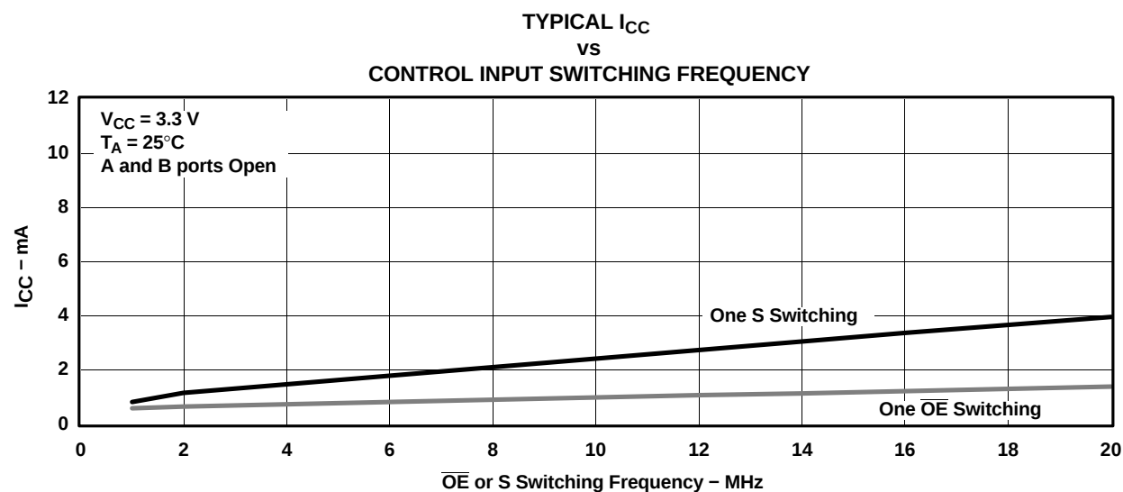
Figure 2. Typical I_{CC} vs \overline{\text{OE}} or S Switching Frequency, V_{CC} = 3.3 \text{ V}
