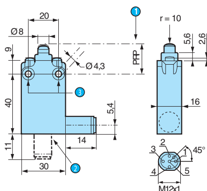
83 870 3/Connector output
