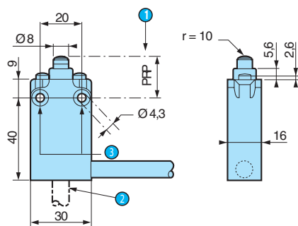
83 870 3/Cable output
