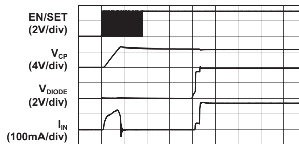
Turn-On to 1.5X Mode (4x30mA Load)
