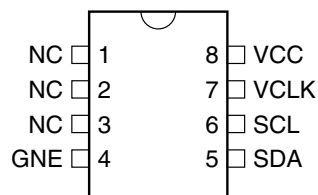
8-pin PDIP
