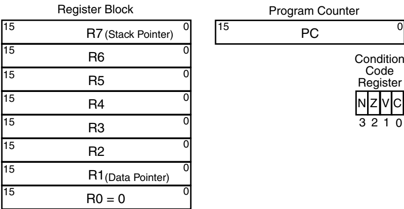
Figure 10-22. Programmer’s Model
