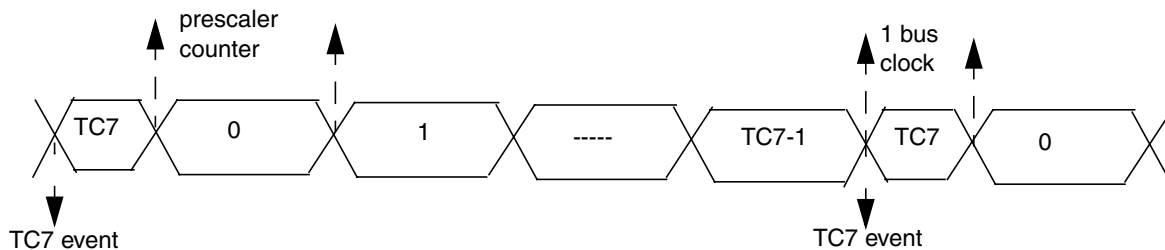
Figure 14-17. The TCNT cycle diagram under TCRE=1 condition
