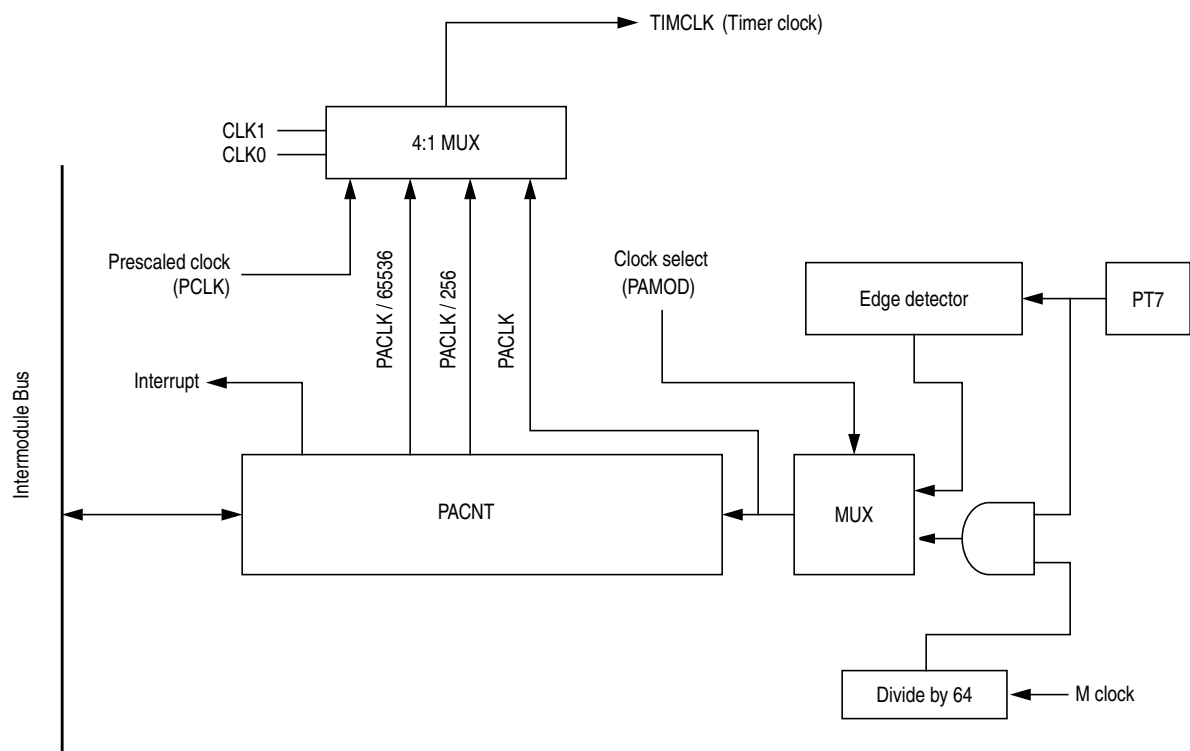
Figure 22-2. 16-Bit Pulse Accumulator Block Diagram
