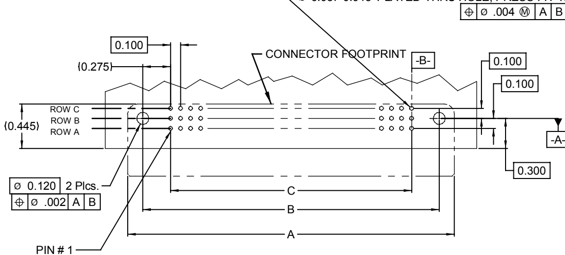
RECOMMENDED P.C.B. HOLE PATTERN
