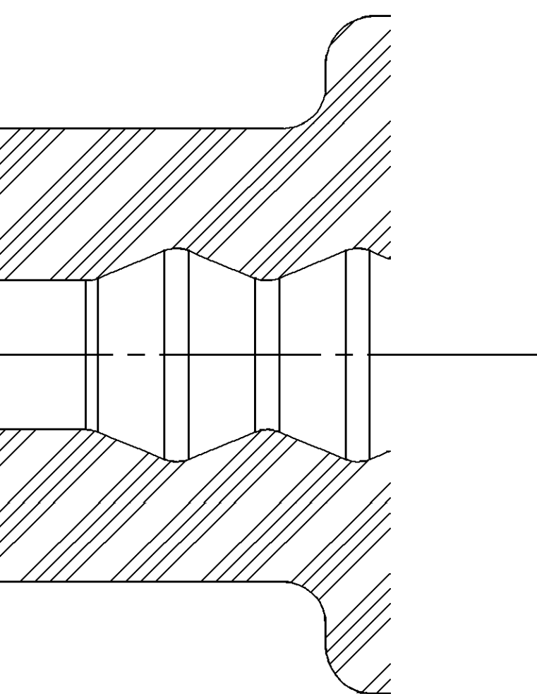
SECTION B-B
