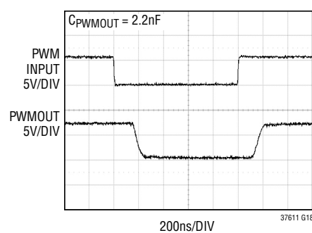
PWMOUT Waveform
