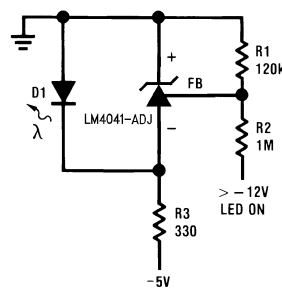
Figure 8-7. Voltage Level Detector
