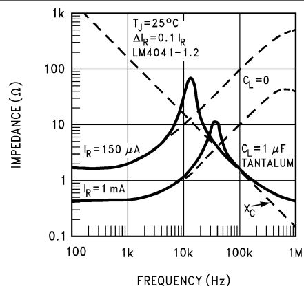
Figure 5-2. Output Impedance vs Frequency
