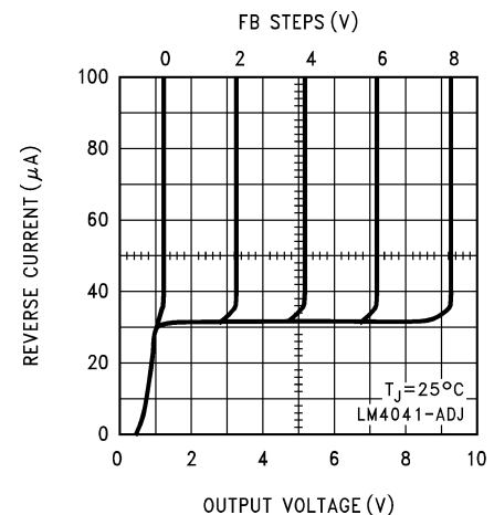
Figure 5-12. Reverse Characteristics
