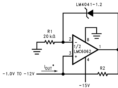
Figure 8-8. Precision 1µA to 1mA Current Sink
