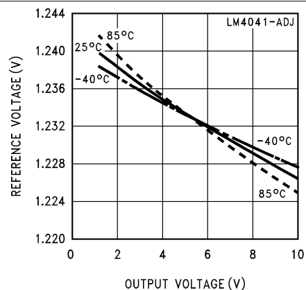
Figure 5-6. Reference Voltage vs Output Voltage and Temperature
