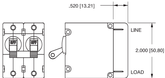
BARRIER FOR UL-RECOGNIZED MULTI-POLE BREAKERS
