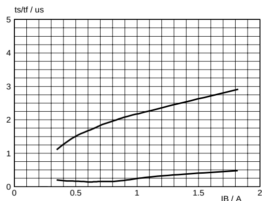
Fig.9. Typical collector storage and fall time. t_s = f(I_B) ; t_f = f(I_B) ; I_C = 5.5 \text{ A} ; T_j = 85^\circ\text{C} ; f = 64 \text{ kHz}
