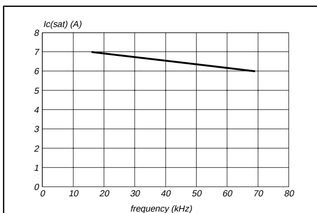
Fig.14. I_{C\text{sat}} during normal running vs. frequency of operation for optimum performance
