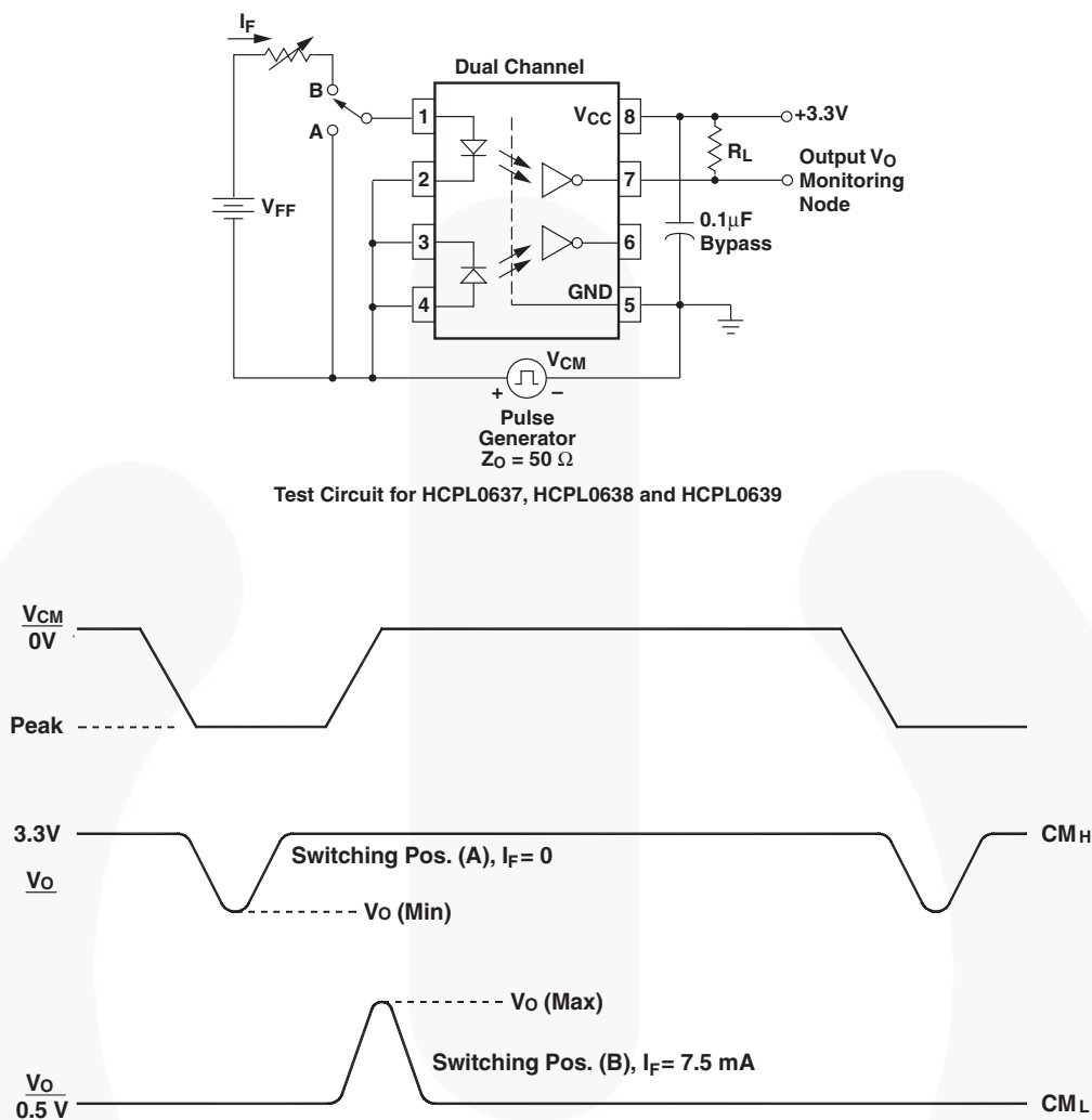
Fig. 23 Test Circuit Common Mode Transient Immunity (HCPL0637, HCPL0638 and HCPL0639)
