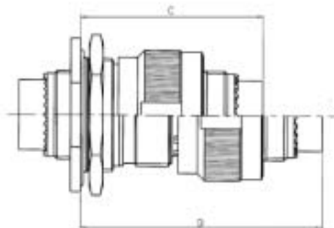
Jam nut receptacle type 7 with plug
