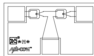
MA4E1319-2
