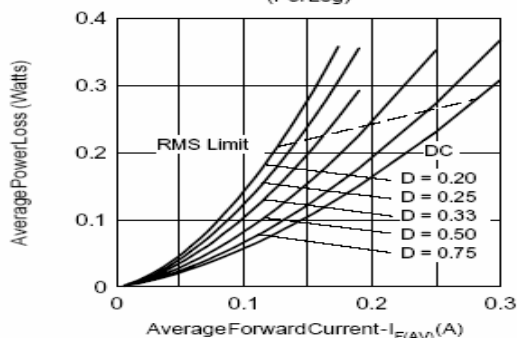
Fig. 4 - Forward Power Loss Characteristics
