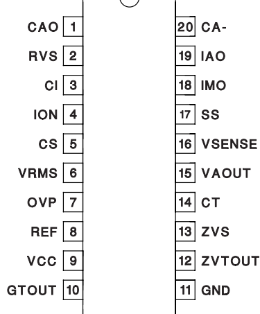
DIL-20 (Top View) J or N Package
