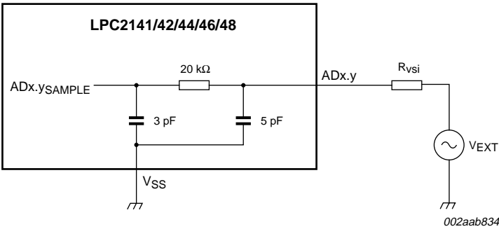
Fig 7. Suggested ADC interface - LPC2141/42/44/46/48 ADx.y pin
