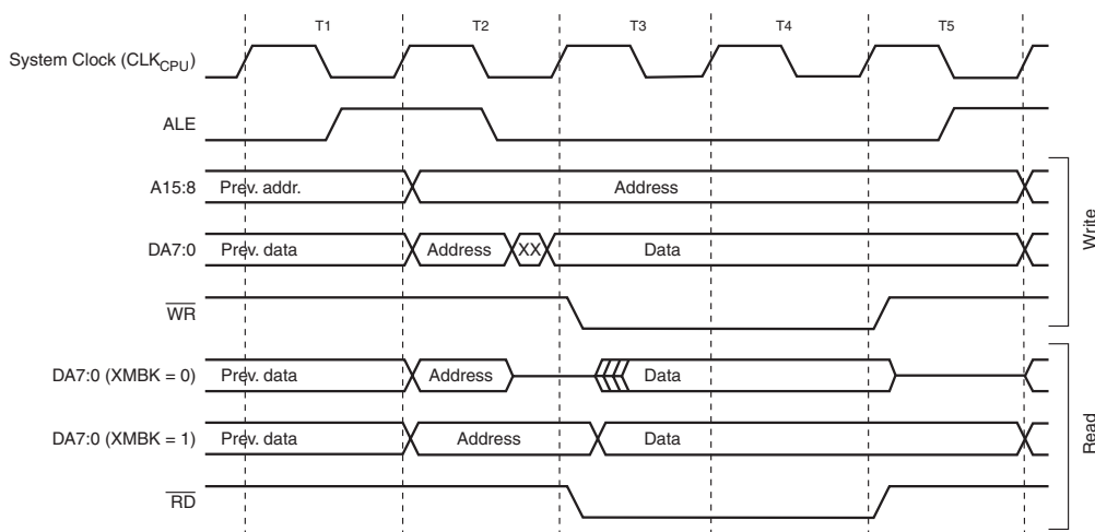
Figure 15. External Data Memory Cycles with SRWn1 = 0 and SRWn0 = 1 (1)
