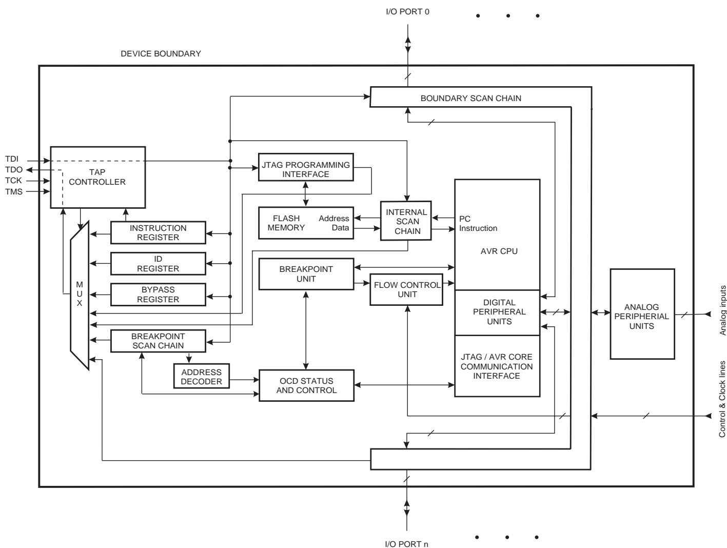
Figure 141. Block Diagram
