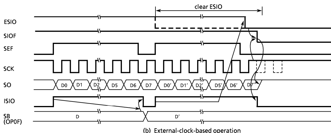
Figure 3-29. Transmit Mode
